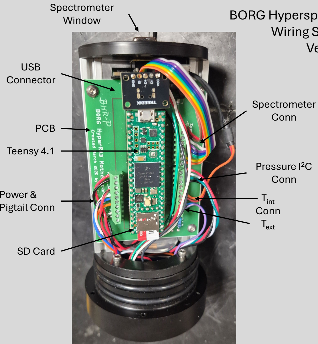
Complete system attached to the base cap
