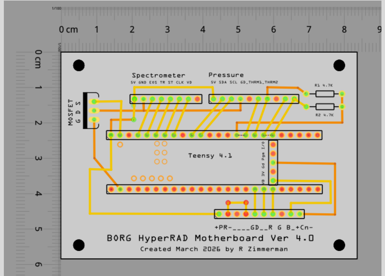
Printed circuit board layout created using Fritzing design software
