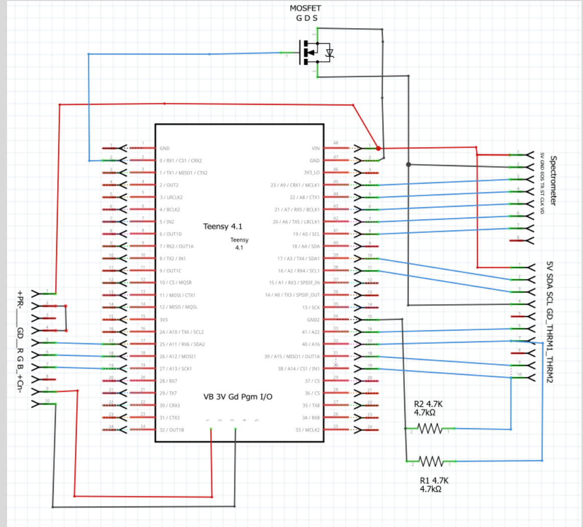
Circuit diagram created using Fritzing design software
